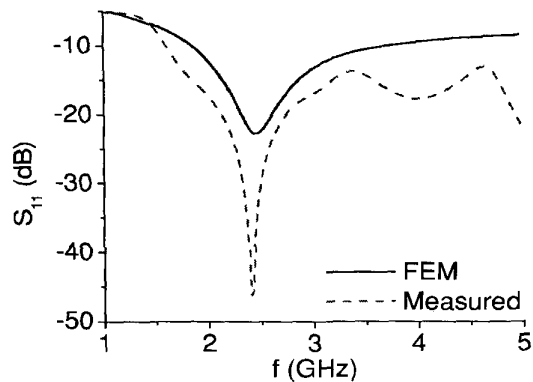
Fig. 4 Comparison of an FEM simulation and VNA measured measurement of the triaxial antenna.
