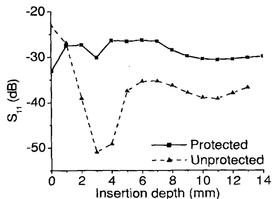
Fig. 5 Insertion depth vs. S_{11} measurements. S_{11} is minimized at 3.5 mm insertion depth.
