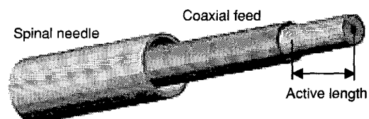
Fig. 1 Coaxial antenna inserted through a biopsy needle.
