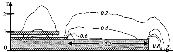
Fig. 2 Normalized electric field magnitudes of a triaxial antenna. Axis dimensions in (mm).
