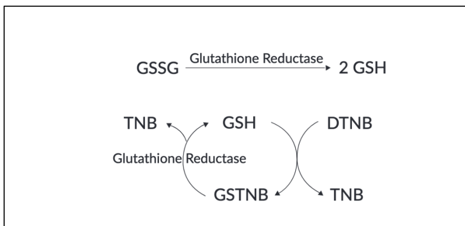
Figure 15: Mechanism of Cayman Chemical Glutathione Recycling Assay. Tietze, 1969
