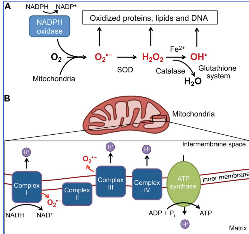
Figure 3: The mitochondrial electron transport chain and production of ROS by electrons escaping coenzyme Q. O_2^{\bullet-} : superoxide; H_2O_2 : hydrogen peroxide; SOD: superoxide dismutase. Bigarella et al. 2014
