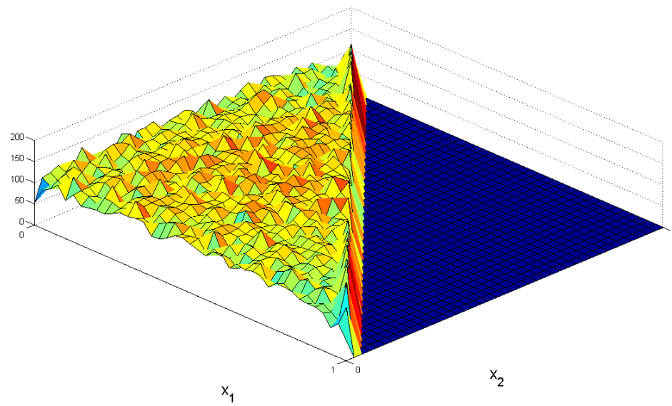
Figure 4.6: Simulation of the uniform distribution for h = 1/40 , T = 5
