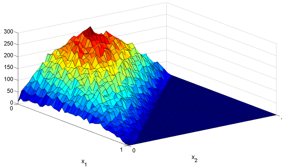
Figure 4.24: Simulation of the distribution with unknown density and h = 1/40 , T = 5
