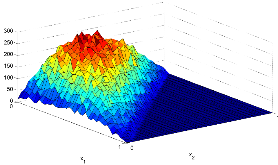
Figure 4.23: Simulation of the distribution with unknown density and h = 1/40 , T = 1
