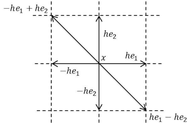
Figure 3.1: Possible transition directions
