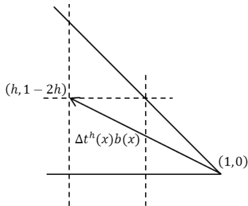
Figure 3.5: Deterministic transition at the vertex.
