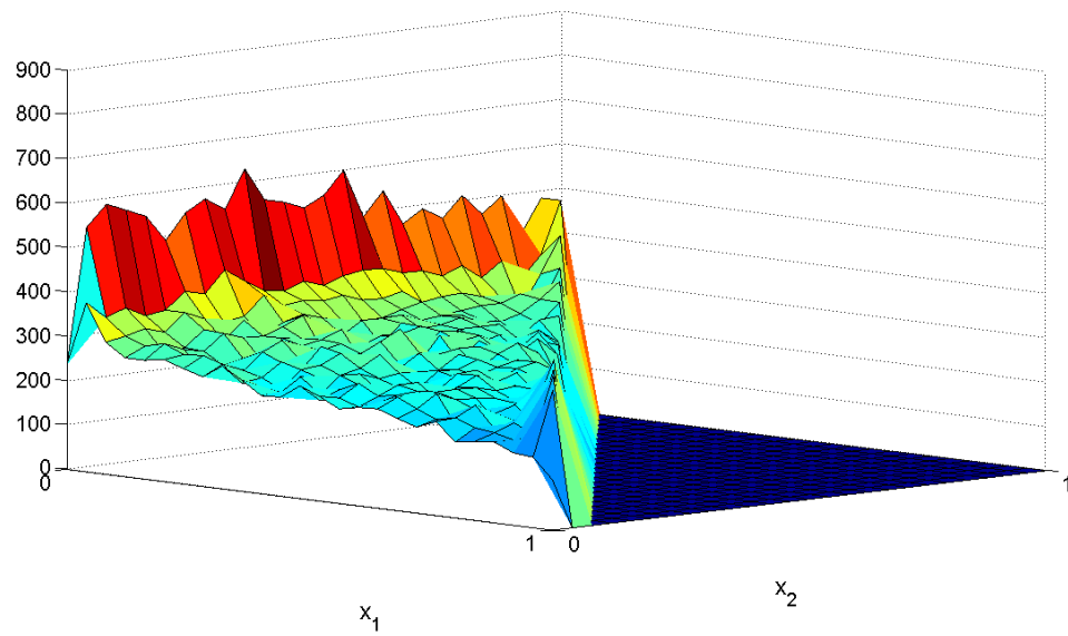
Figure 4.10: Simulation of the Dirichlet distribution with h = 1/25 , T = 0.5
