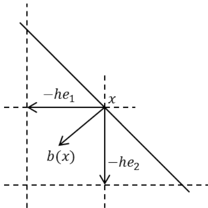
Figure 3.3: The algorithm can be used if b_1(x) \leq 0 and b_2(x) \leq 0 .
