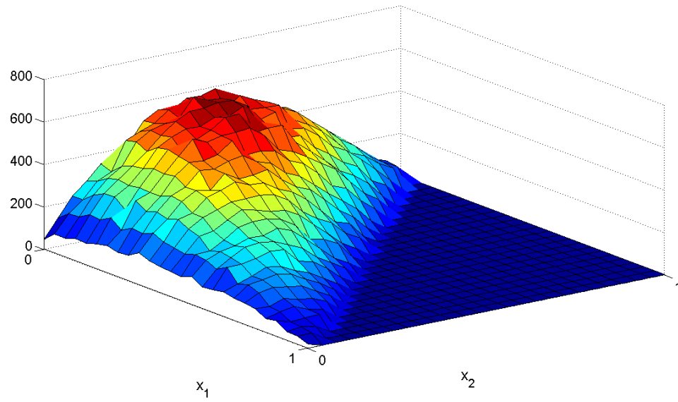
Figure 4.21: Simulation of the distribution with unknown density and h = 1/25 , T = 5
