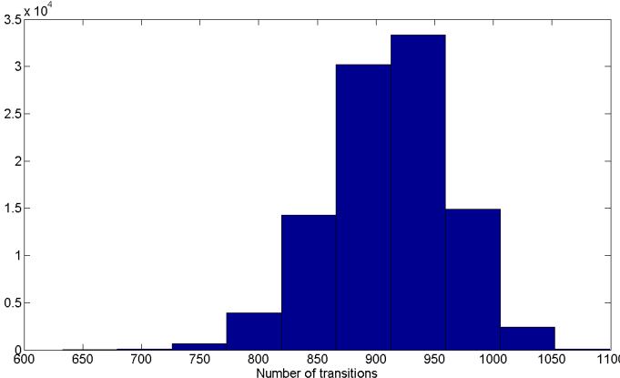
Figure 4.2: Distribution of the number of transitions for h = 1/25
