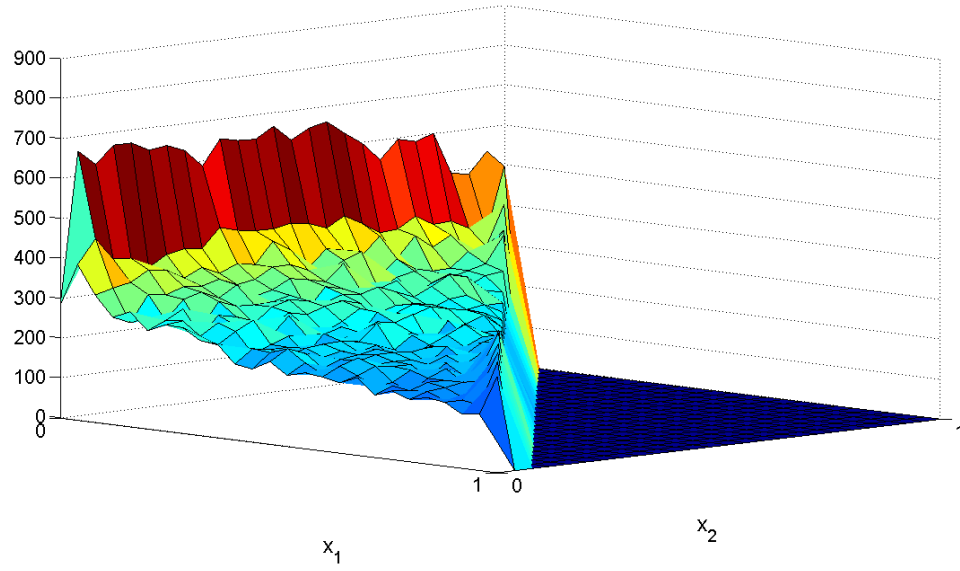
Figure 4.11: Simulation of the Dirichlet distribution with h = 1/25 , T = 1
