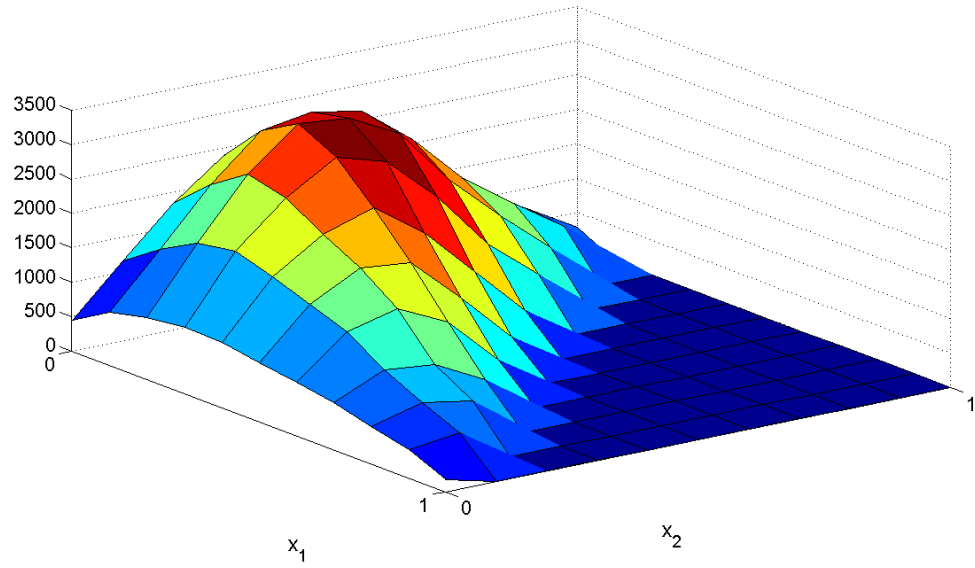
Figure 4.17: Simulation of the distribution with unknown density and h = 1/10 , T = 1
