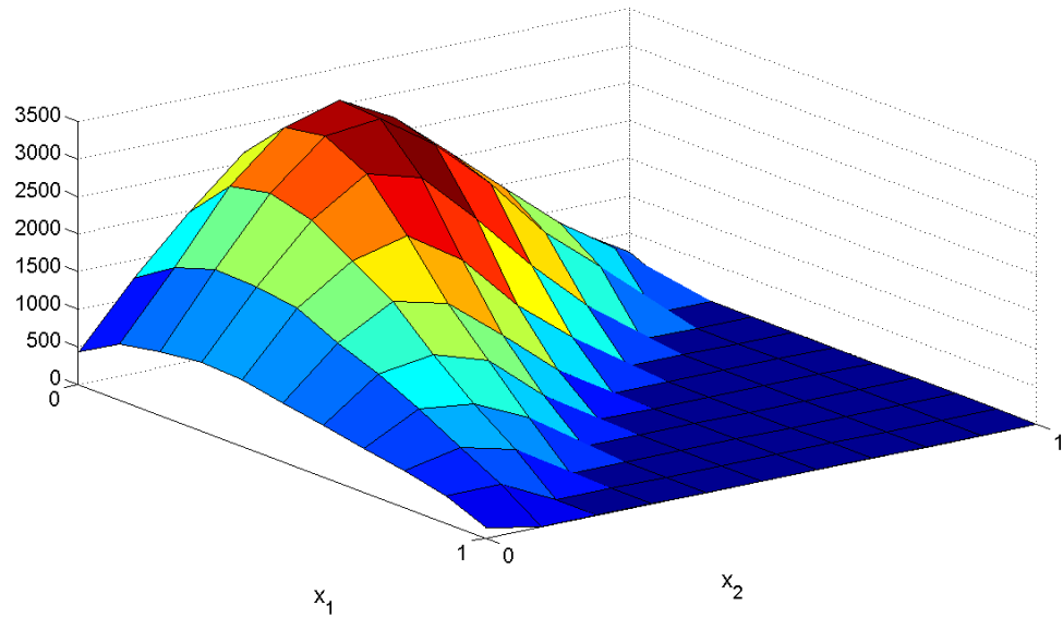
Figure 4.18: Simulation of the distribution with unknown density and h = 1/10 , T = 5
