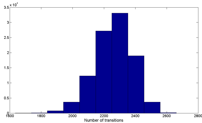
Figure 4.3: Distribution of the number of transitions for h = 1/40
