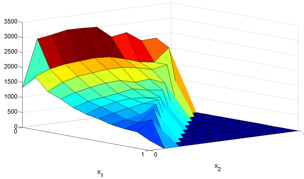
Figure 4.9: Simulation of the Dirichlet distribution with h = 1/10 , T = 5
