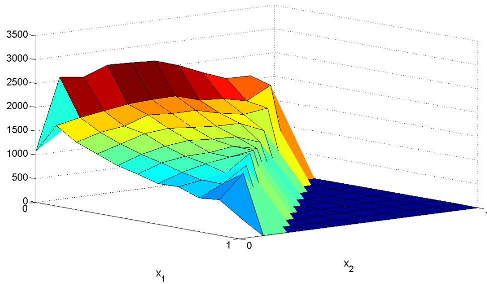
Figure 4.8: Simulation of the Dirichlet distribution with h = 1/10 , T = 1
