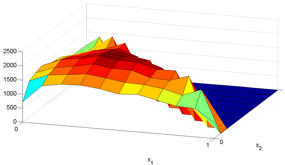
Figure 4.4: Simulation of the uniform distribution for h = 1/10 , T = 5
