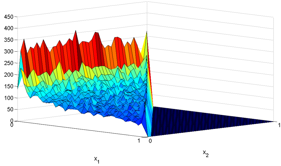
Figure 4.14: Simulation of the Dirichlet distribution with h = 1/40 , T = 1
