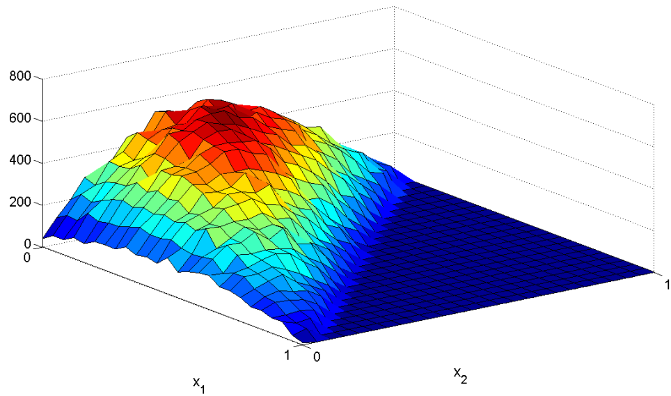
Figure 4.20: Simulation of the distribution with unknown density and h = 1/25 , T = 1
