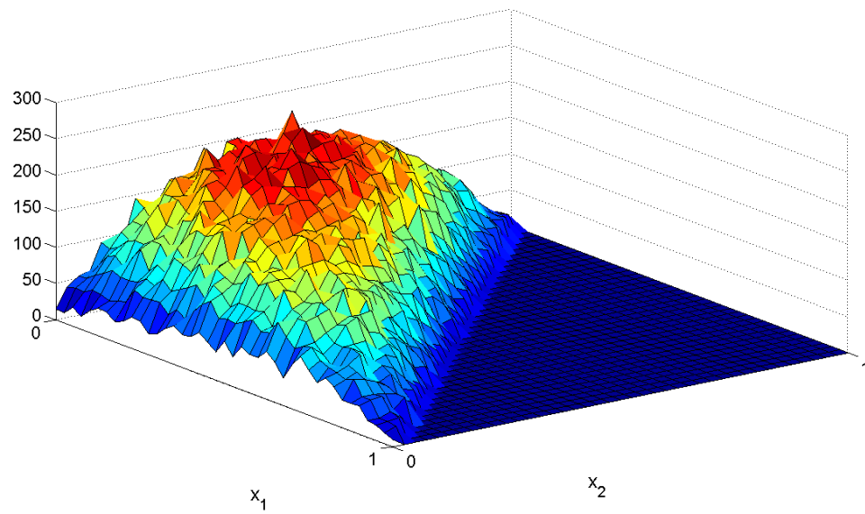
Figure 4.22: Simulation of the distribution with unknown density and h = 1/40 , T = 0.5
