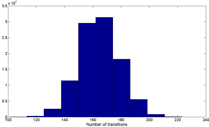
Figure 4.1: Distribution of the number of transitions for h = 1/10
