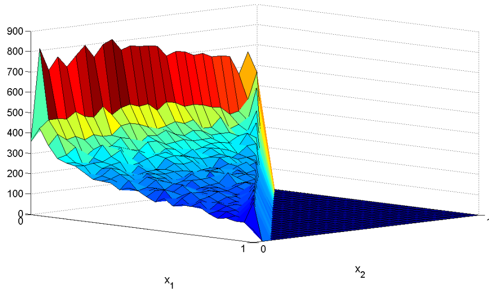
Figure 4.12: Simulation of the Dirichlet distribution with h = 1/25 , T = 5
