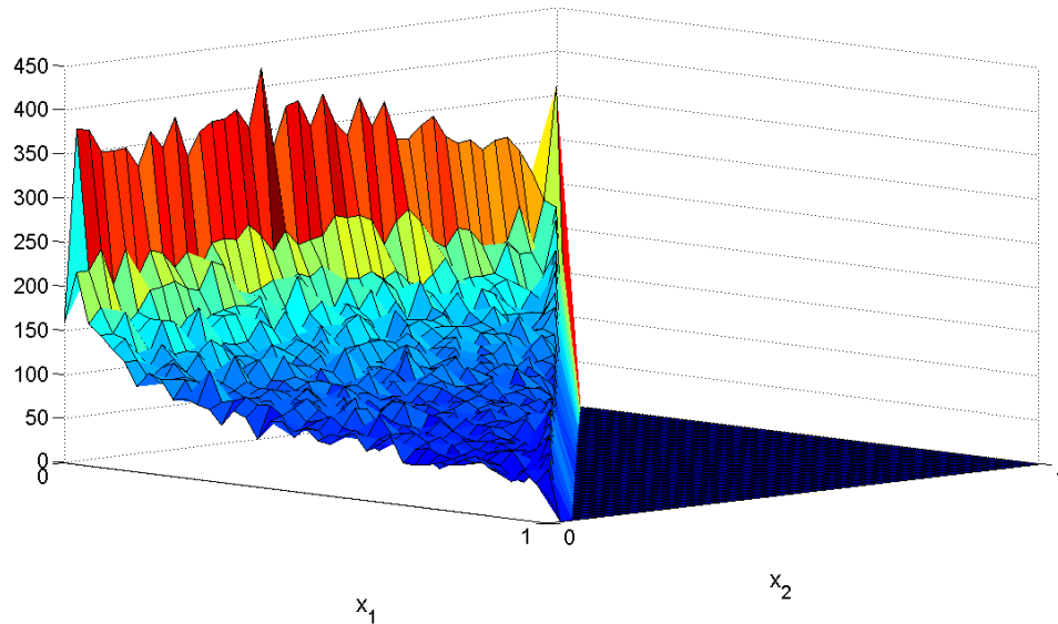
Figure 4.15: Simulation of the Dirichlet distribution with h = 1/40 , T = 5
