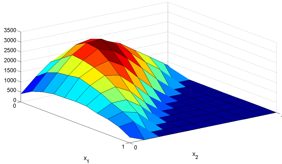
Figure 4.16: Simulation of the distribution with unknown density and h = 1/10 , T = 0.5
