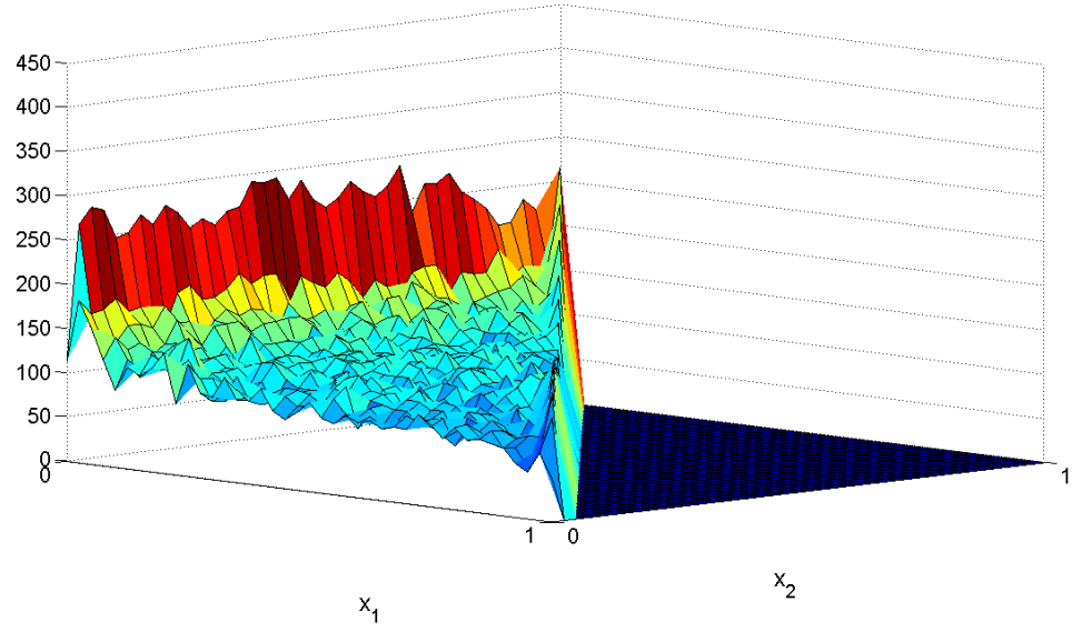
Figure 4.13: Simulation of the Dirichlet distribution with h = 1/40 , T = 0.5
