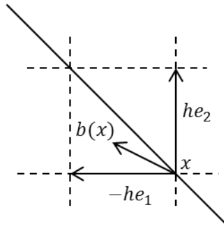
Figure 3.2: Leaving the triangle by a transition along he_2
