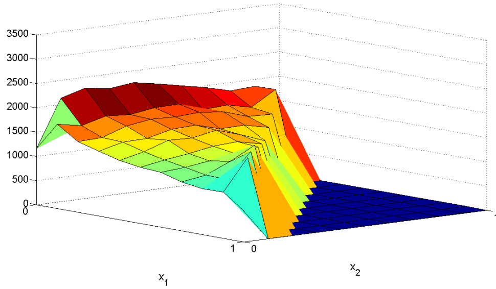
Figure 4.7: Simulation of the Dirichlet distribution with h = 1/10 , T = 0.5
