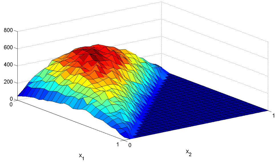
Figure 4.19: Simulation of the distribution with unknown density and h = 1/25 , T = 0.5
