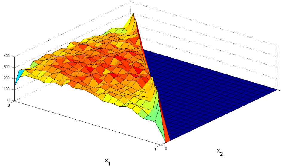
Figure 4.5: Simulation of the uniform distribution for h = 1/25 , T = 5
