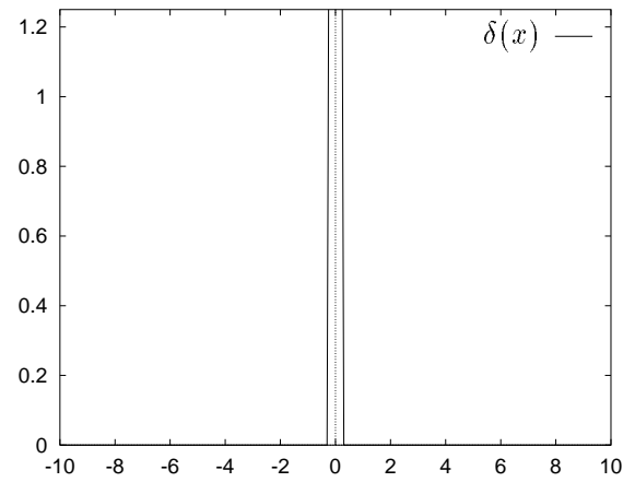
Figure 3: The Dirac delta function \delta(x)
