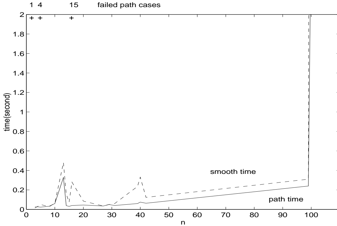
Figure 13: Smooth with Newton preprocessor versus PATH 2.7 for Small MCP
