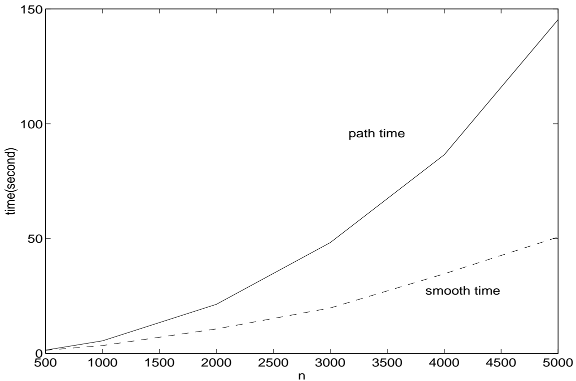
Figure 10: Smooth versus PATH for Optimal Control Problem(bert_oc.gms)
