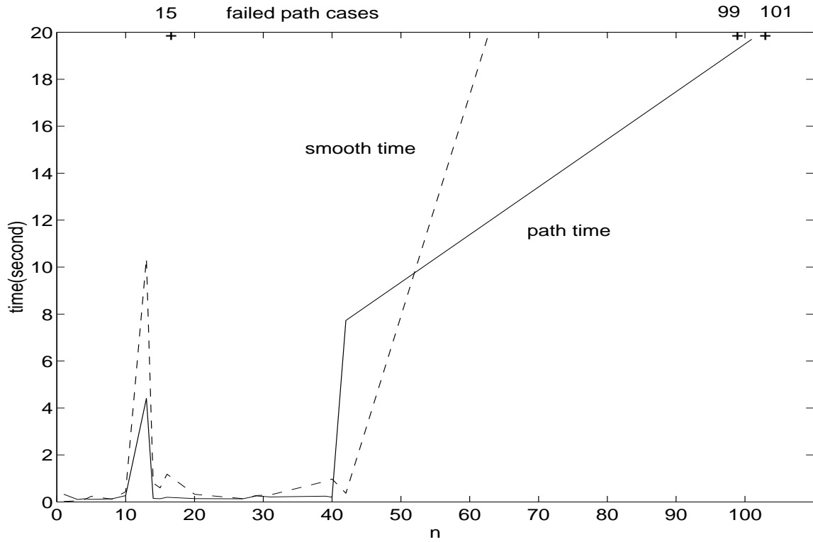
Figure 9: Smooth versus PATH for Small MCP
