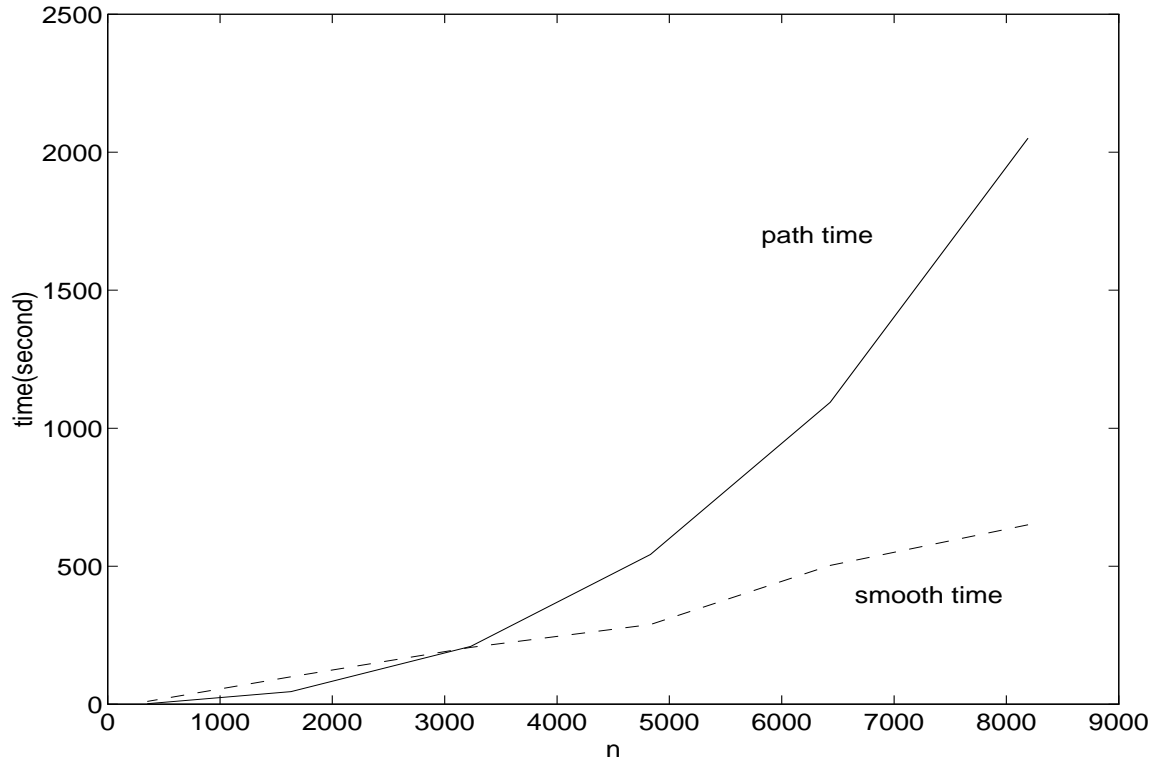
Figure 11: Smooth versus PATH for Optimal Control Problem(opt_cont.gms)
