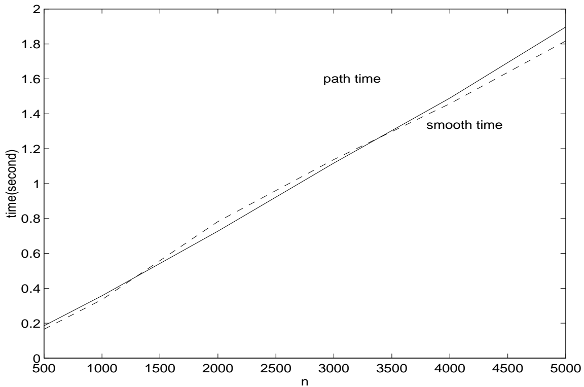
Figure 14: Smooth with Newton preprocessor versus PATH 2.7 for Optimal Control Problem(bert_oc.gms)
