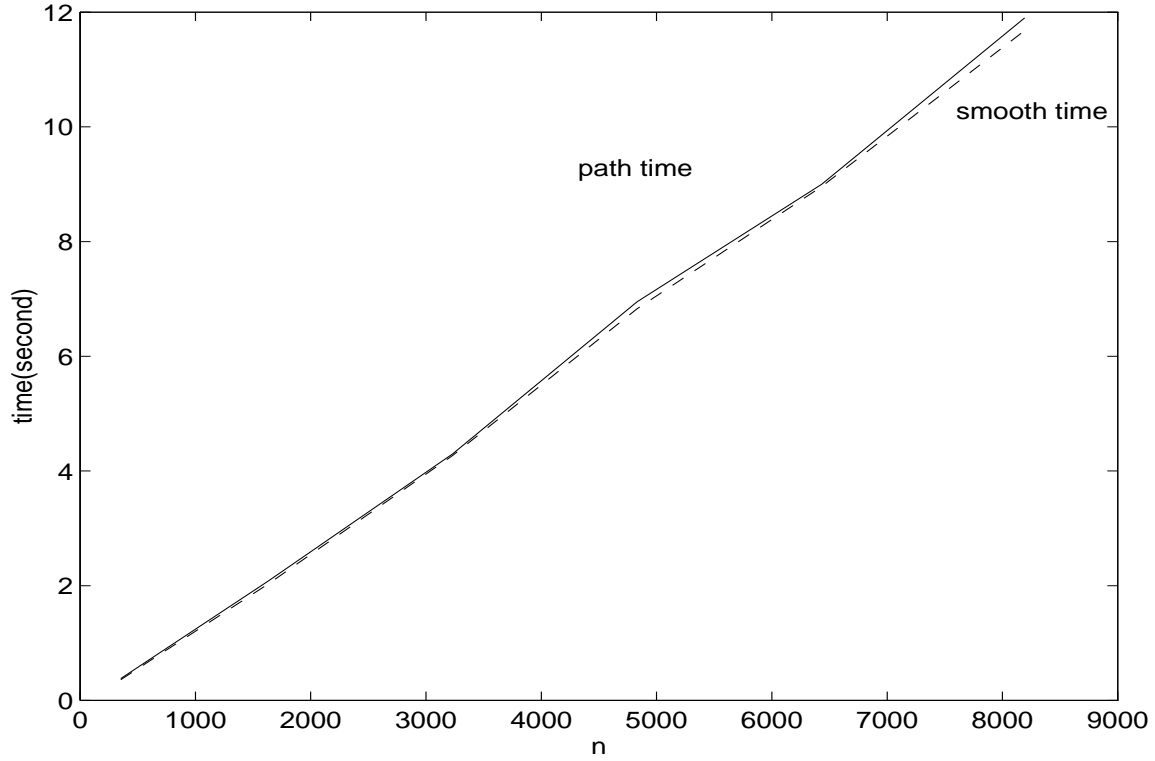
Figure 15: Smooth with Newton preprocessor versus PATH 2.7 for Optimal Control Problem(opt_cont.gms)
