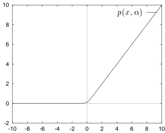
Figure 4: The p function p(x, \alpha) = x + \frac{1}{\alpha} \log(1 + e^{-\alpha x}) with \alpha = 5
