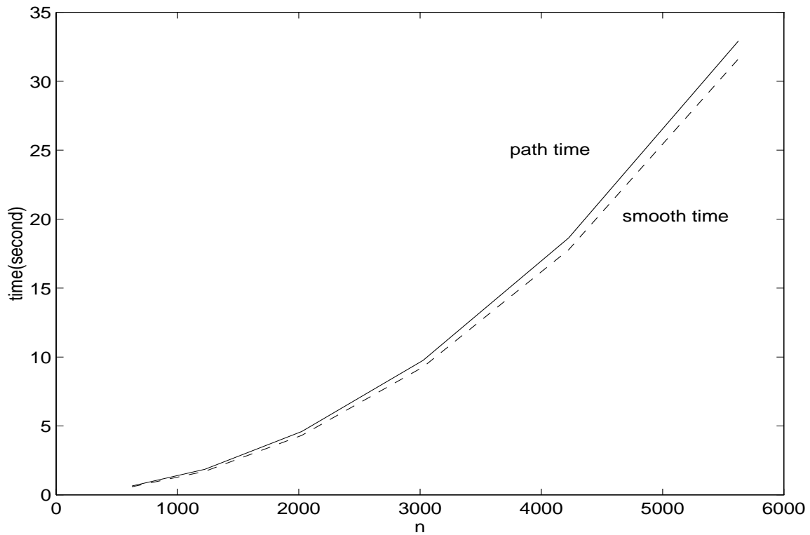
Figure 16: Smooth with Newton preprocessor versus PATH 2.7 for Obstacle Problems
