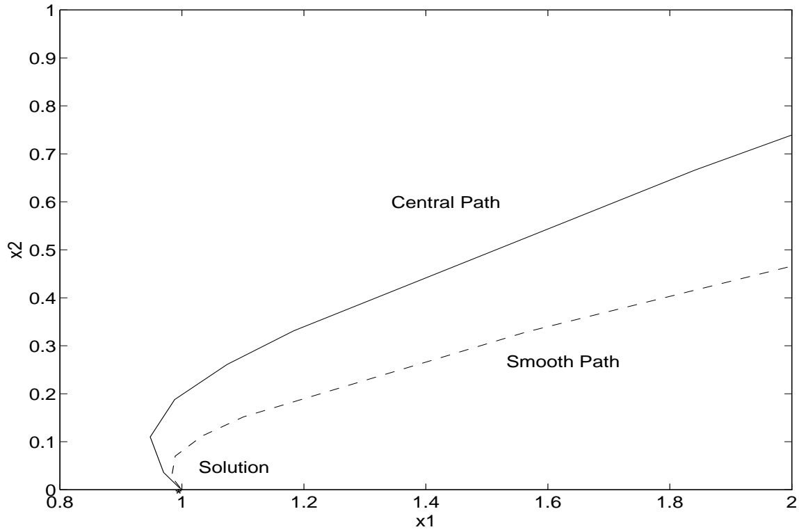
Figure 7: Comparison of the interior smooth path generated by an exact solution of the smooth nonlinear equation (10) versus the central path for Example 5.1
