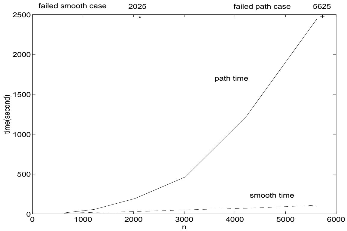
Figure 12: Smooth versus PATH for Obstacle Problems
