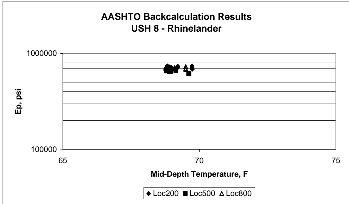
Figure 3.3.2 Pavement Modulus vs Mid-Depth Temperature for USH8-Rhinelande Corehole Locations
