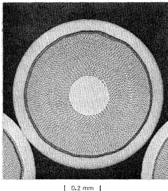
Fig. 1a. Micrograph of a typical MJR conductor cross section. Proceeding out from center, the components are bronze core, bronze and Nb expanded metal spiral wrap, Nb and Ta diffusion barrier, and Cu.
