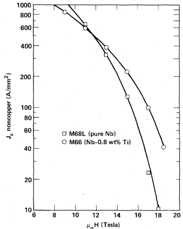
Fig. 3. Critical current density (in non-copper area) for a typical sample containing Ti additions compared with a typical sample with pure Nb cores. The enhancement in J_c at higher fields with Ti additions is quite significant.
