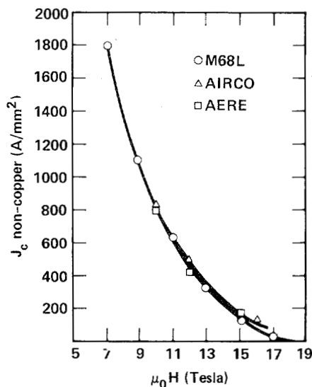
Fig. 5. Comparison of J_c values for MJR-process material with several results for optimized, conventional, bronze-process material. Filament cores in all cases are pure Nb.
