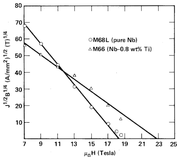
Fig. 4. A plot of J_c^{1/2} B^{1/4} vs. \mu_0 H , which provides an estimate of H_{c2} by extrapolation to J_c^{1/2} B^{1/4} = 0 , after Kramer. 5
