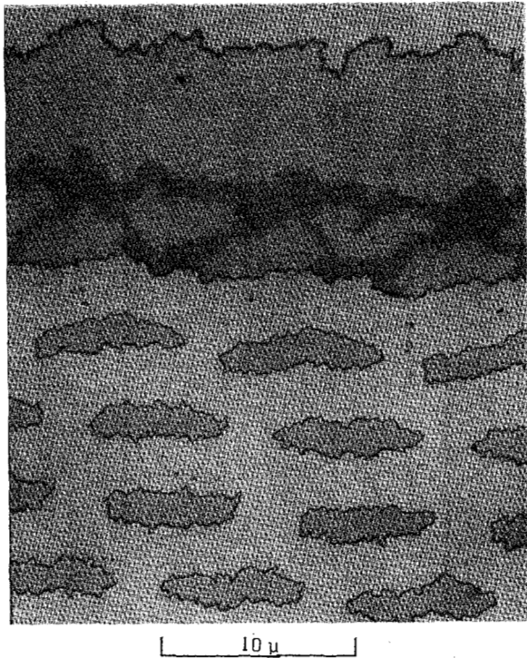
Fig. 1b. Enlarged micrograph showing outer filaments and diffusion barrier. Dark layer in diffusion barrier is Ta. Filaments maintain the rectangular cross section of the starting material throughout processing.
