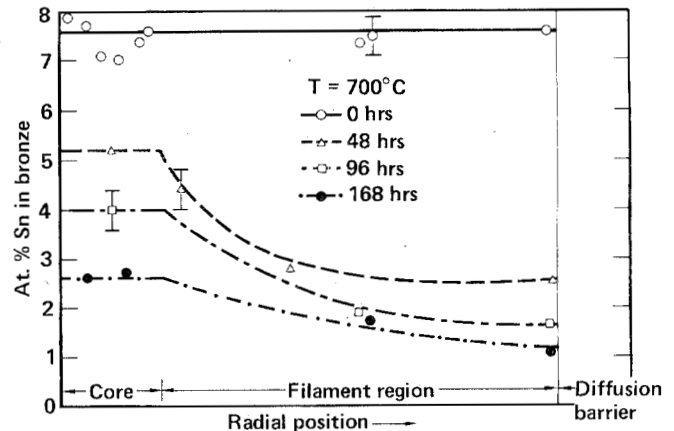
Fig. 6. Scanning Auger Microprobe results showing the evolution of Sn profiles in the bronze matrix following various heat treatments.
