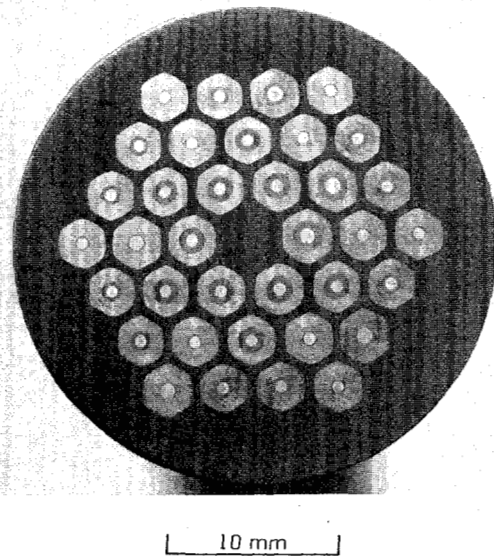
Fig. 2. Micrograph of HFTF-type conductor cross section after extrusion and drawing.
