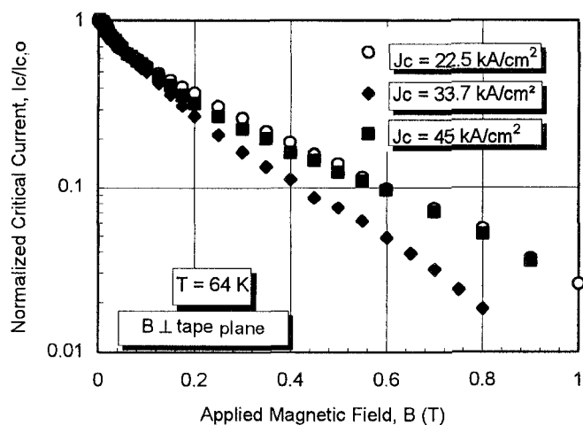
Fig. 5. The retention of critical current relative to the self field value at 64 K for three rolled 85 filametary conductors with J_c values of 22.5, 33.7, and 45 \text{kA/cm}^2 , showing independence of connectivity and flux pinning.
