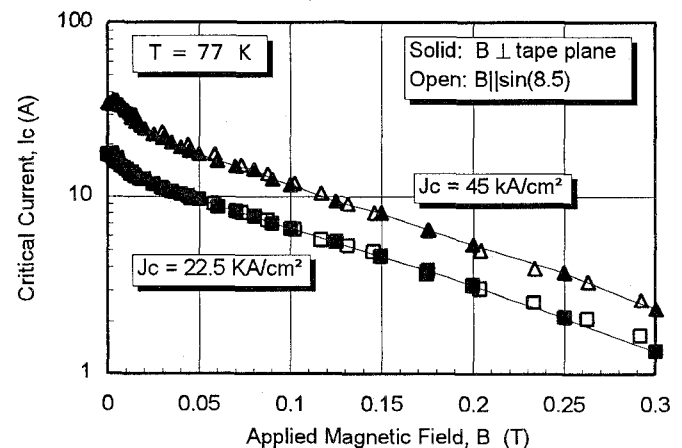
Fig. 4. The dependence of I_c on magnetic field for two 85 filament s for the two principal field orientations at 77 K, showing weak link reduction. The B \parallel field magnitude has been scaled by \sin(8.5) to account for the fitted misorientation of the grains.
