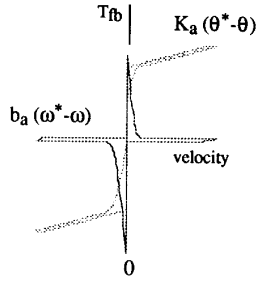
Fig. 9. Breakdown of feedback torque error components.
