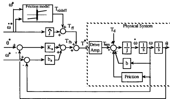
Fig. 11. Nonlinear decoupling state feedforward friction compensation technique.
