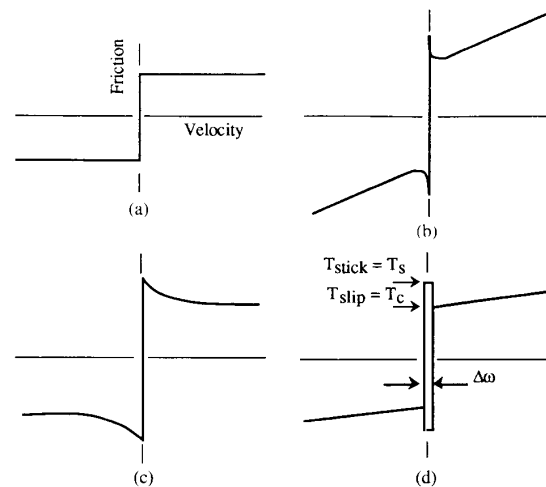
Fig. 1. Velocity-dependent friction models: (a) Coulomb friction model; (b) including stiction and viscous damping; (c) exponential model; (d) causal model with stick region.
